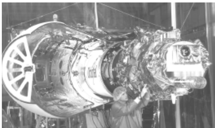
Orbital's DART integrated with the Pegasus launch vehicle
